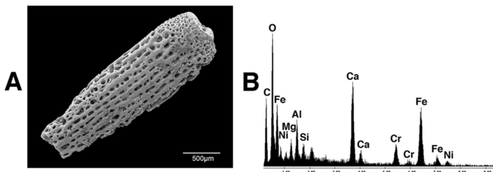
Fig. 17. High Mg carbonate fragment. A: SEM image of submarine fossil. B: X-ray analysis of surface of fossil near metal contamination from stainless steel sieve
