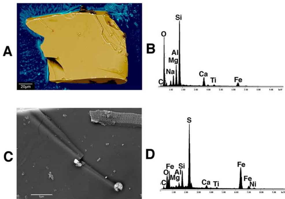
Fig. 20. Pyrite spherule indenting basaltic glass. A: SEM image of entire grain. Pyrite spherule is colored red. B: X-ray analysis of the composition of the glass. C: Close up of iron sulfide spherule indenting glass. The pyrite is following a single track. The offset of the track is an optical illusion. D: X-ray analysis of the composition of the spherule
