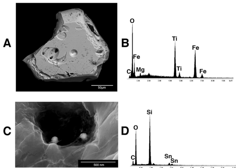
Fig. 10. Unusual components of layer C. A: Ilmenite grain with unusual craters on its surface. B: X ray analysis of ilmenite. C: Sn-rich silicate spherules in hole in quartz grain. D: X-ray analysis of spherules
