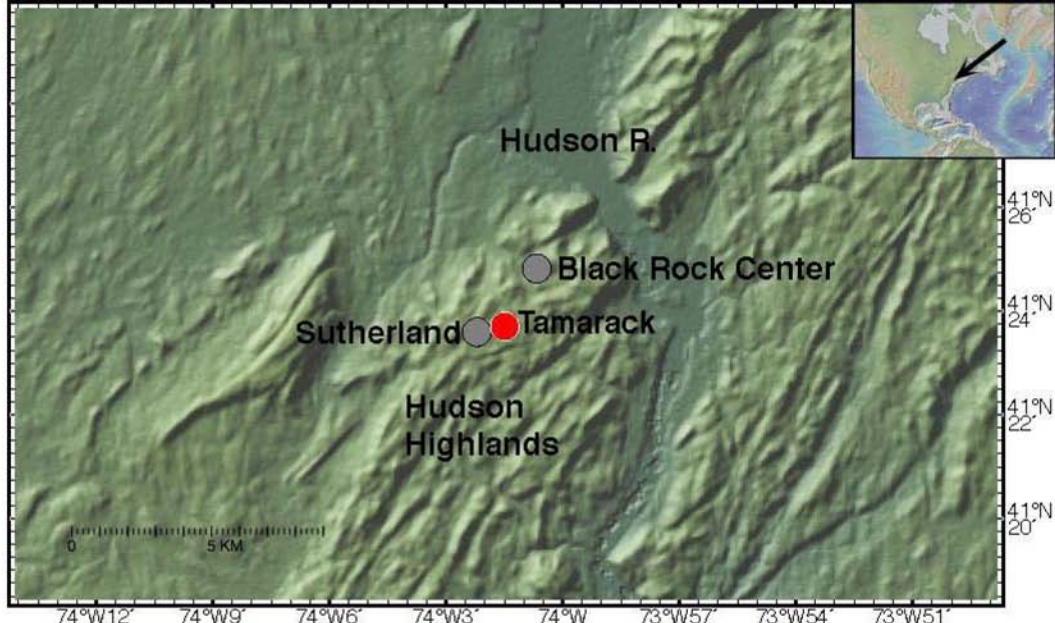
Fig. 1. Location map. Inset. Location of Black Rock Forest relative to east coast of North America. Large map: Red circle: Location of Tamarack Pond. Gray circles: Locations of Sutherland Pond and central administration building of Black Rock forest in Cornwall, NY. Black Rock forest is in the Hudson Highlands just west of the Hudson River. Image from Geomapapp.
