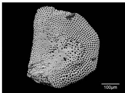
Fig. 13. Marine carbonate fossil. A: SEM image of marine fossil. B: X-ray analysis of composition of fossil. Note that there is a strong Mg peak, consistent with either aragonite or high Mg calcite. The carbonate contains about 26 mol% Mg
