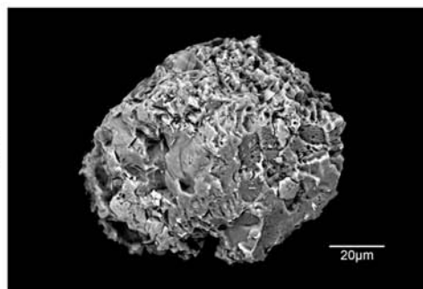
Fig. 15. Glass Grains. A: SEM image of grain with conchoidal fracture. B: X-ray analysis of composition of the grain in A. C: SEM image of grain with conchoidal fracture. Parts of the grain appear vesiculated. D: X-ray analysis of the composition of grain in C
