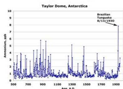
Fig. 6. Ammonium values in ice core samples. A: Ammonium values in the GISP2 ice core from Greenland [24, 34]. B: Ammonium values in the Taylor dome ice core from Antarctica [25]
