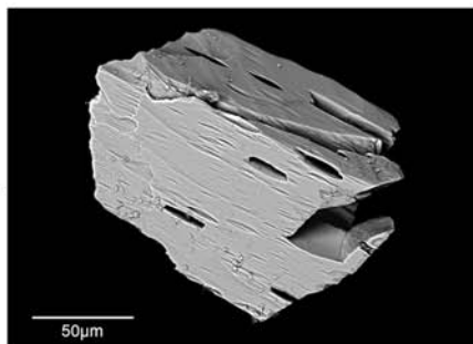
Fig. 14. Basaltic glass with lens-shaped fractures. A: SEM image of black basaltic glass with lens shaped fractures. B: X-ray analysis of composition of the glass
