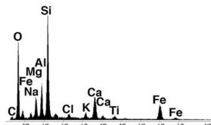
Fig. 14. Basaltic glass with lens-shaped fractures. A: SEM image of black basaltic glass with lens shaped fractures. B: X-ray analysis of composition of the glass
