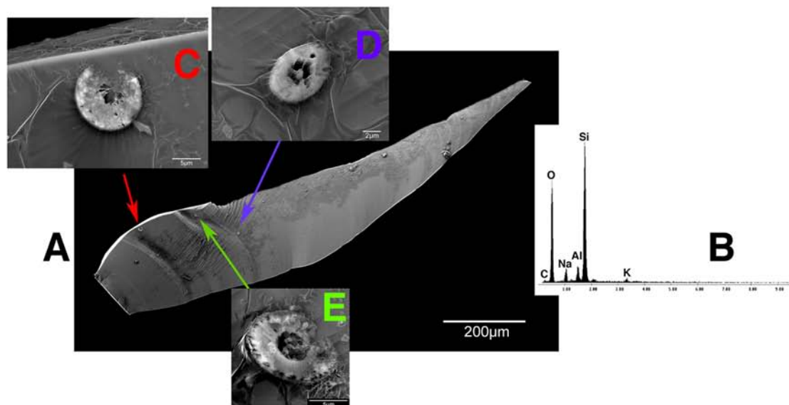
Fig. 22. Glass shard with embedded silicified coccoliths. A. SEM image of entire glass shard. B. X-ray analysis of glass shard. C, D and E. Embedded silicified coccoliths
