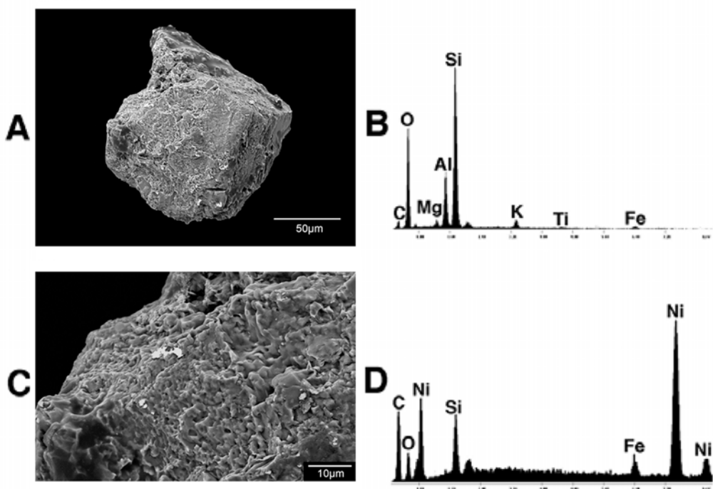
Fig. 16. Metal on Clear Grain. A. SEM backscatter image of entire grain. B. X-ray analysis of composition of grain matrix. C. SEM backscatter detail of grain showing melted, vesiculated surface and bright material of higher atomic number splashed on surface. D. X-ray analysis of composition of bright material (includes contribution from surrounding matrix)
