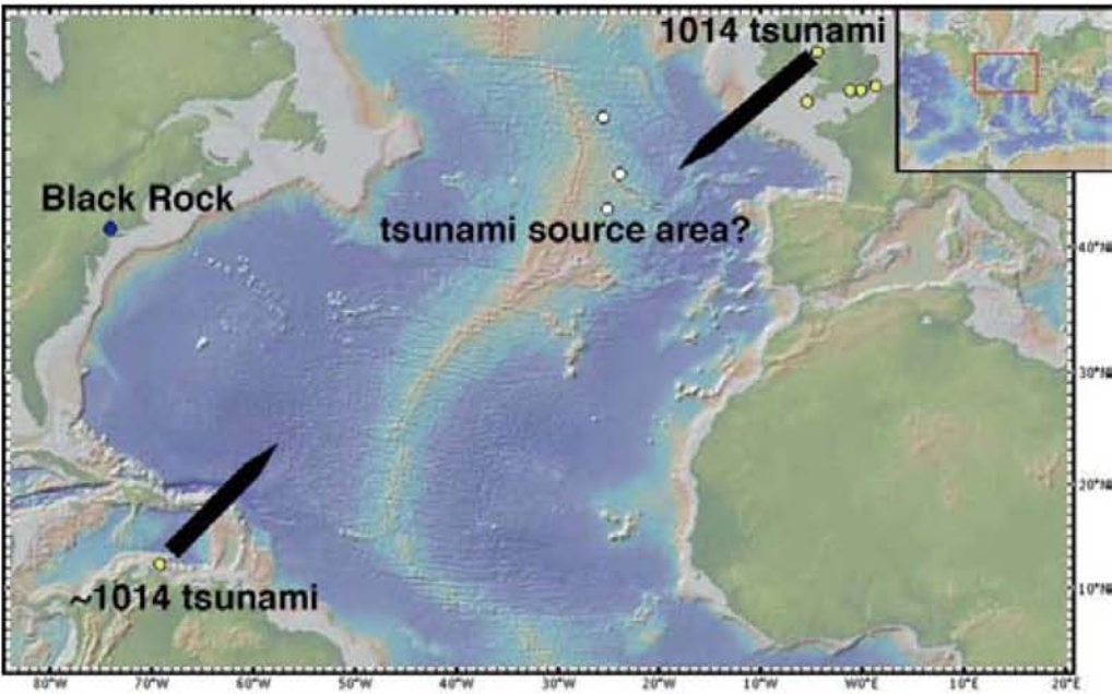
Fig. 5. Proposed source area of transported layer in Black Rock forest and locations of 1014 A.D. or circa 1014 A.D. layers White circle: source area with glauconite and radiolarians in marine sediment that also has young basalt close to the surface. Blue circle: Location of Black Rock Forest. Yellow circles: Locations of tsunami deposits that are circa 1014 A.D. (Caribbean) or have an exact calendar year date of September 28, 1014 A.D. (Great Britain). Arrows: Inferred direction to tsunami source derived from the elongation direction of tsunami boulder deposits.
