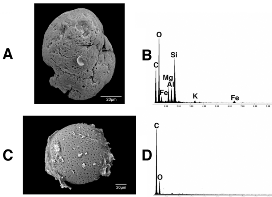
Fig. 3. Glauconite microfossil cast and C rich spherule. A. Microfossil cast composed of glauconite clay. The cast is green in color. B. X-ray analysis (EDAX) of the composition of the microfossil cast. C. Perfectly round, vesicular spherule. D. X-ray analysis (EDAX) of the composition of the spherule
