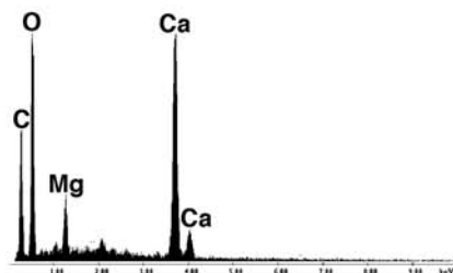
Fig. 13. Marine carbonate fossil. A: SEM image of marine fossil. B: X-ray analysis of composition of fossil. Note that there is a strong Mg peak, consistent with either aragonite or high Mg calcite. The carbonate contains about 26 mol% Mg
