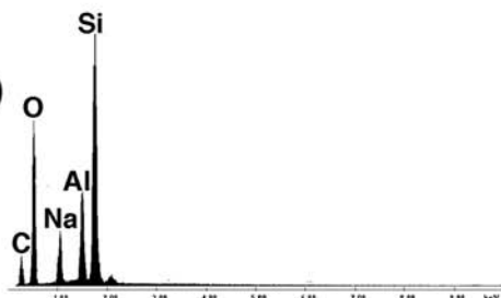
Fig. 15. Glass Grains. A: SEM image of grain with conchoidal fracture. B: X-ray analysis of composition of the grain in A. C: SEM image of grain with conchoidal fracture. Parts of the grain appear vesiculated. D: X-ray analysis of the composition of grain in C
