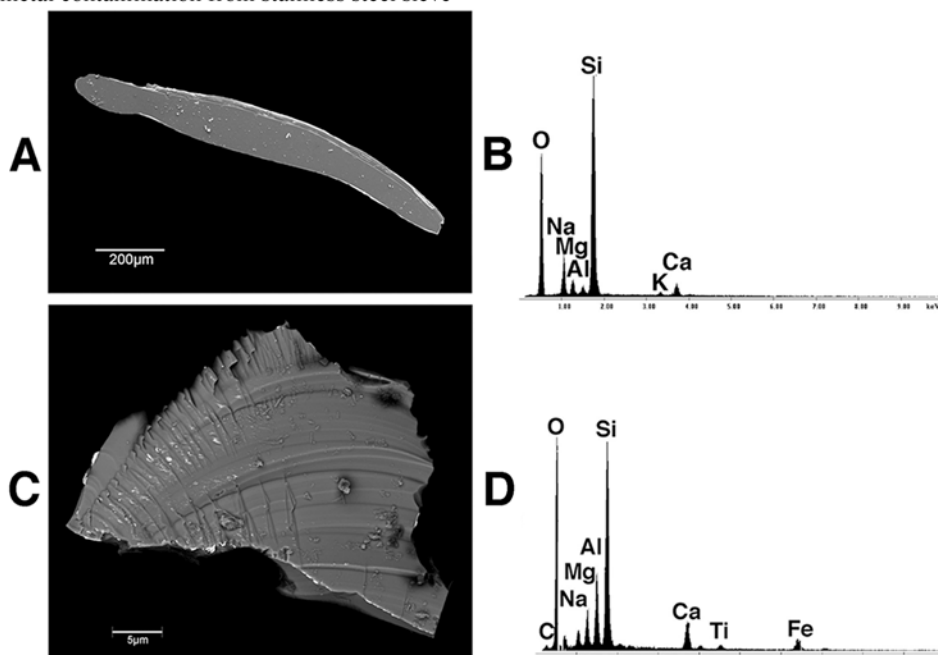
Fig. 18. Conchoidally fractured grains that appear to be glass. A: SEM image of optically clear glass shard. B: X-ray analysis of the composition of the glass shard. C: Optically clear greenish grain with conchoidal fracture and gouges. D: X-ray analysis of the composition of C
