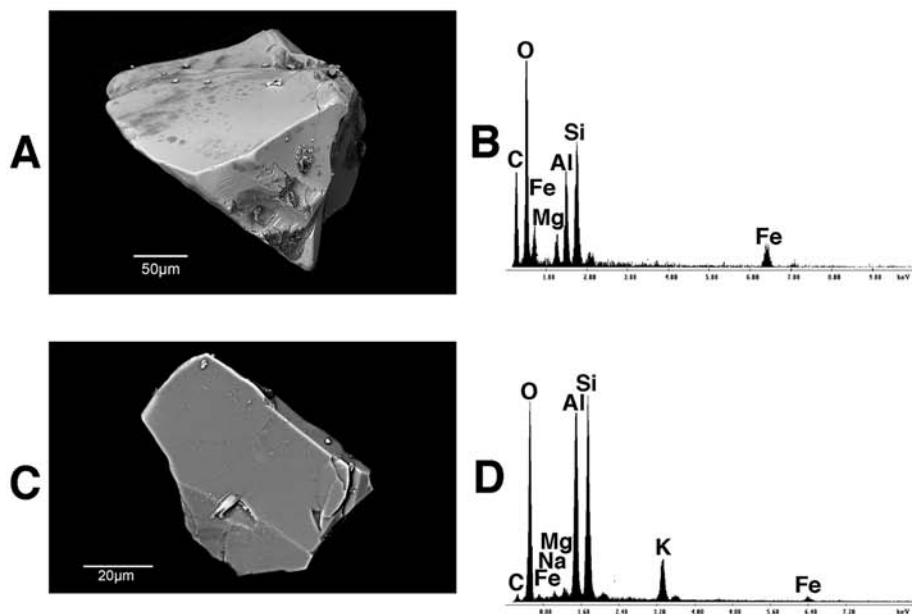
Fig. 19. Possible mineral grains. A: Optically clear pink grain with conchoidal fracture. B: X-ray analysis of the composition of the grain in A. C: Optically clear grain with section peeled back like sardine can. D: X-ray analysis of the composition of the grain in C
