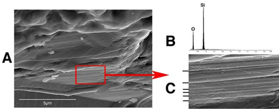
Fig. 12. Possible shocked quartz grain (unpolished). A: SEM image of surface of the grain. Three directions of planar features are visible. The spacing between the planar fractures is less than a micron, one defining characteristic of shock lamellae. B: X-ray analysis of the composition of the grain. C: Enlargement of the best-resolved planar features in Fig. A. Edges of the best resolved planar features are delineated by lines on the left side of the image. The height of the image is equal to a distance of 3.1 micrometers. The planar features in this image have a spacing of much less than 1 micrometer and thus are clearly PDFs resulting from shock metamorphism [19] rather than metamorphic deformation features
