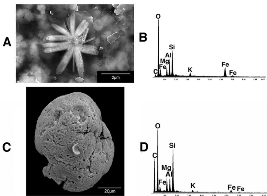
Fig. 9. Comparison of glauconite in two different forms. A: Glauconite rosette on top surface of rock fragment from Layer C. B: X-ray analysis of glauconite rosette to left. C: Microfossil cast composed of glauconite from layer A. D: X-ray analysis of glauconite cast to left. Note in particular the three iron peaks in both X-ray analyses
